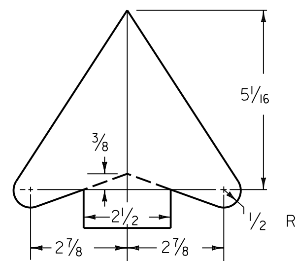
ARROW HEAD DETAIL
