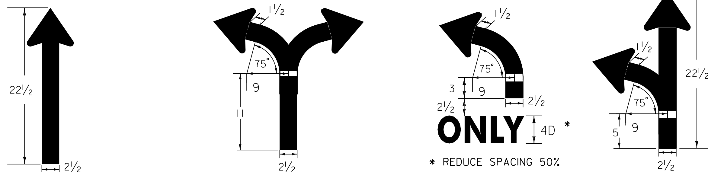
ARROW CONFIGURATION DETAILS
