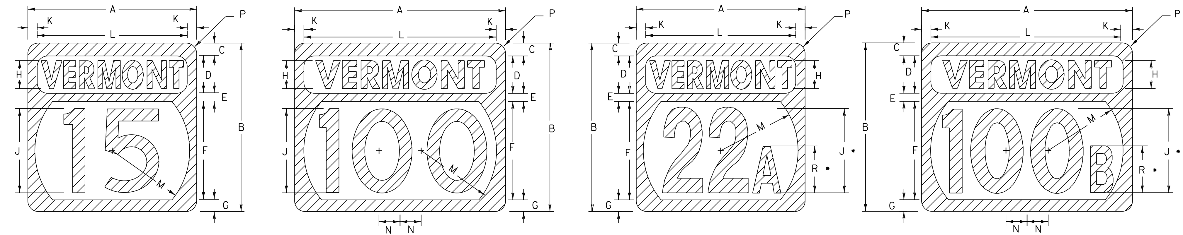
1 OR 2 DIGIT STATE ROUTE MARKER WITHOUT BORDER
