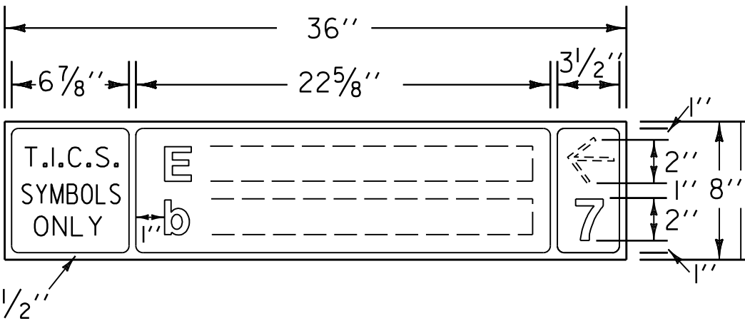
HALF-SIZED DIRECTIONAL SIGN DETAIL
