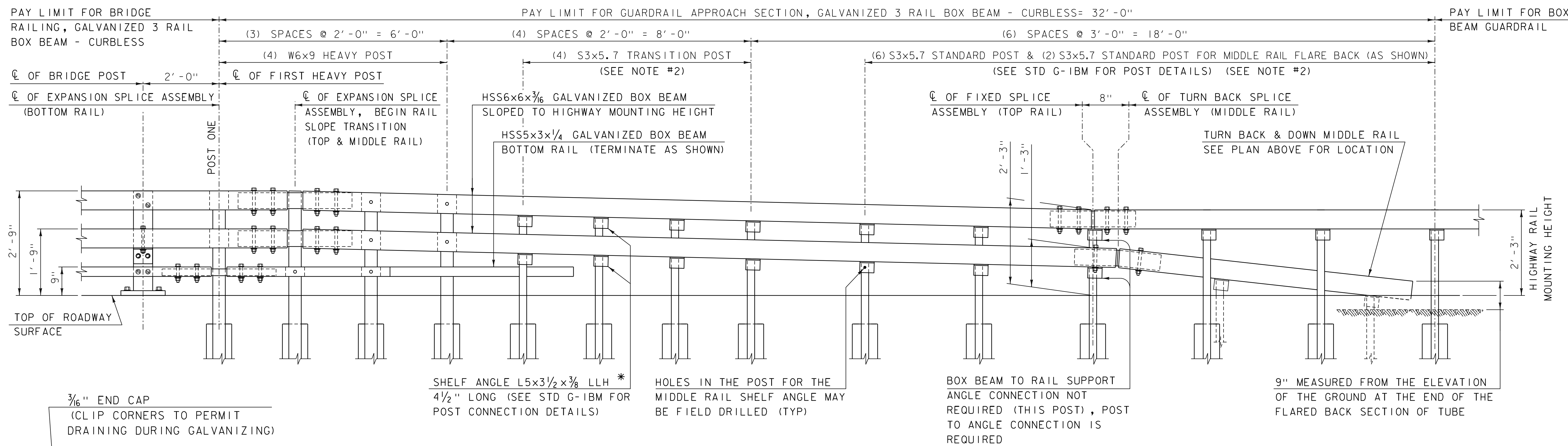
3 RAIL BOX BEAM ELEVATION
