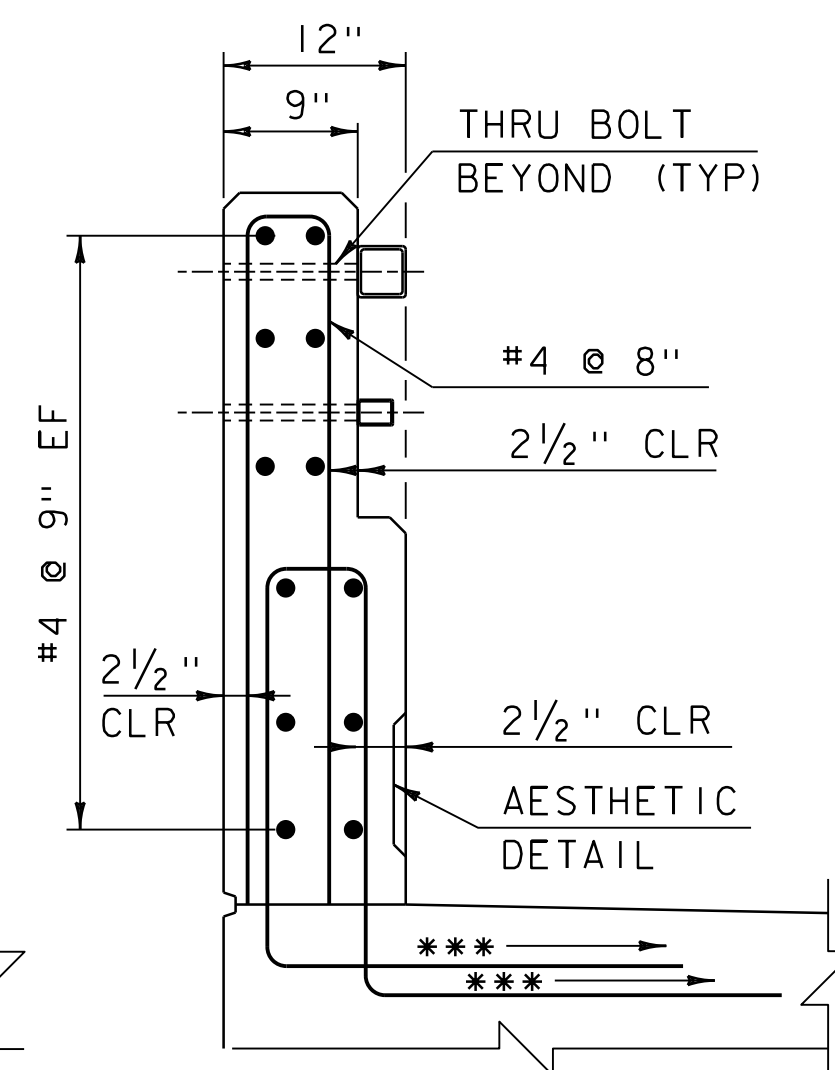
SECTION B-B
