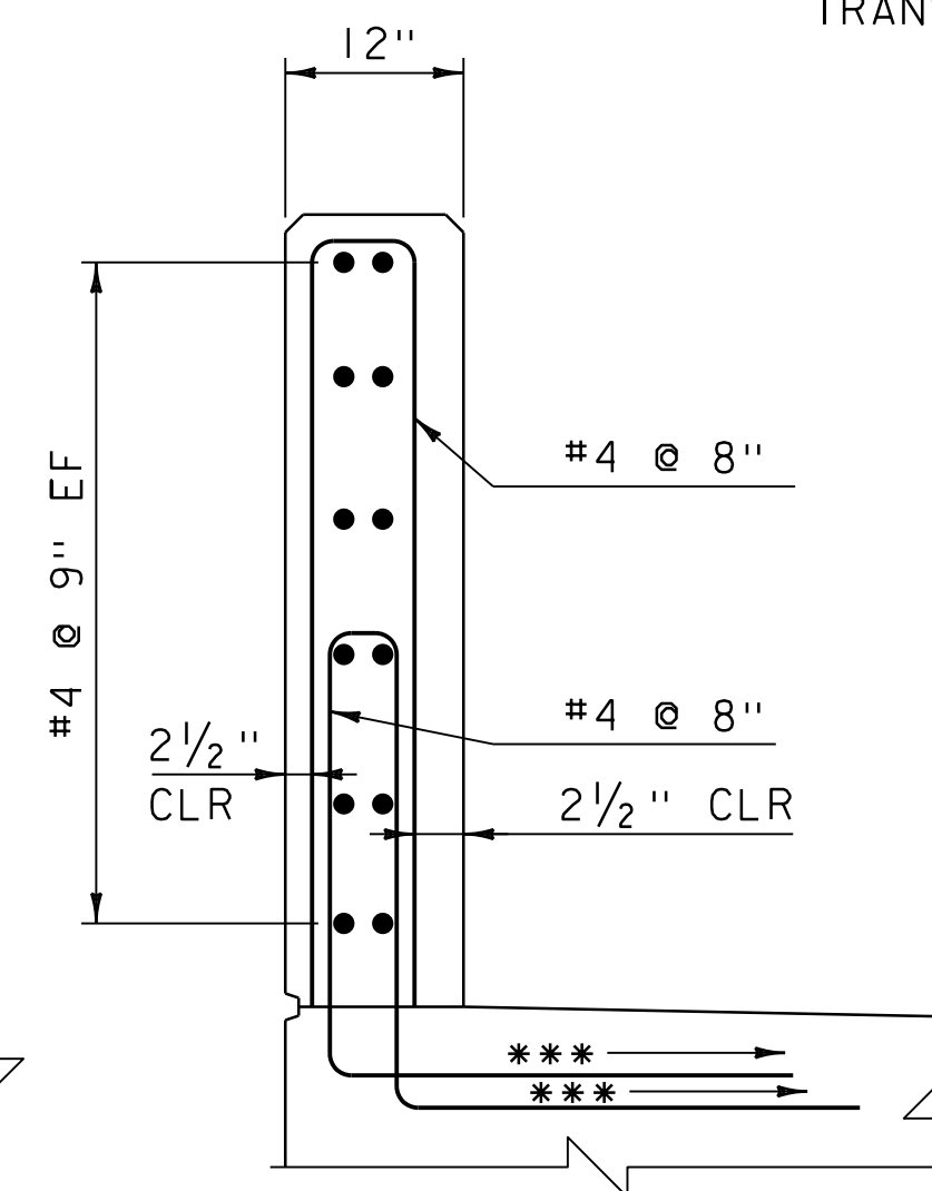
SECTION C-C
