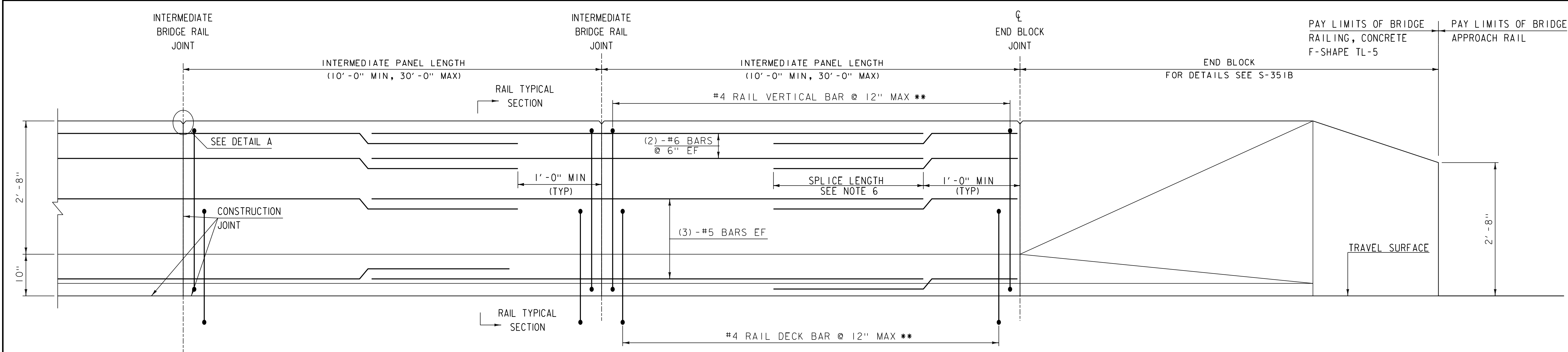
BRIDGE RAIL ELEVATION NTS
