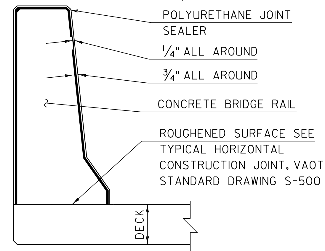
BRIDGE RAIL JOINT SECTION
