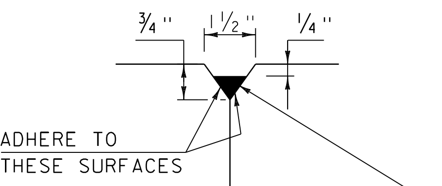
BRIDGE RAIL JOINT SECTION
