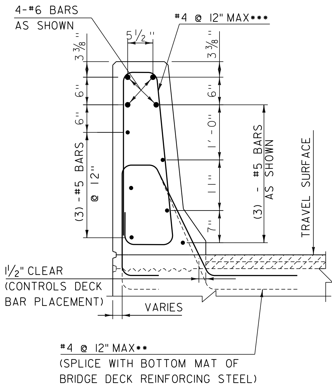
RAIL REINFORCING SECTION
