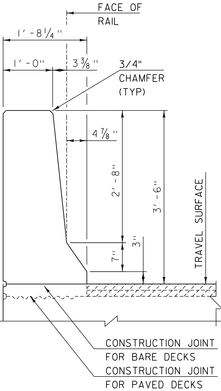
RAIL TYPICAL SECTION
