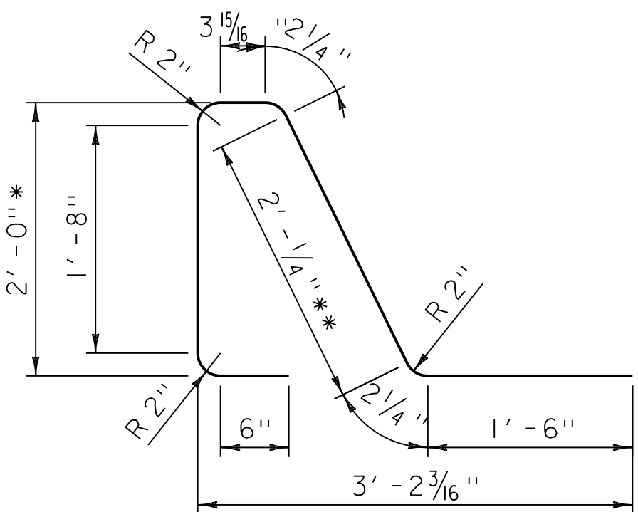
#4 RAIL DECK BAR
