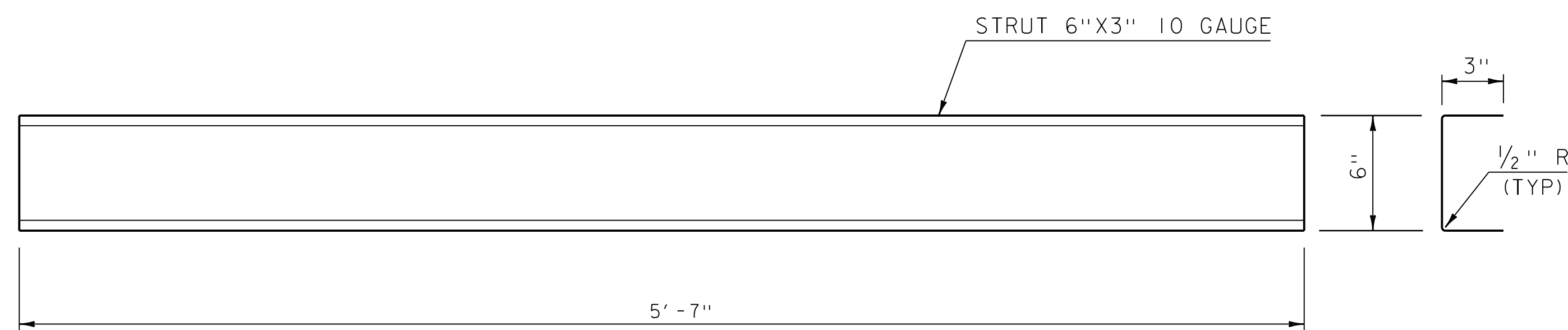
YOKE DETAIL
