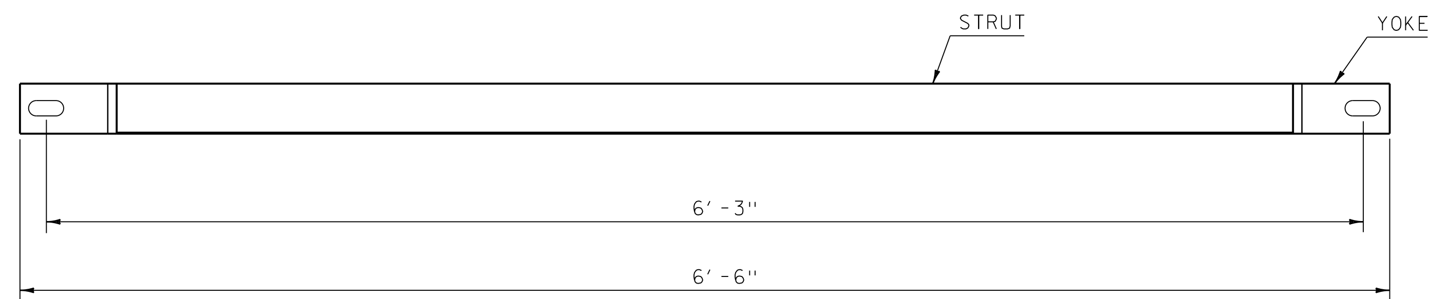
TOP VIEW
