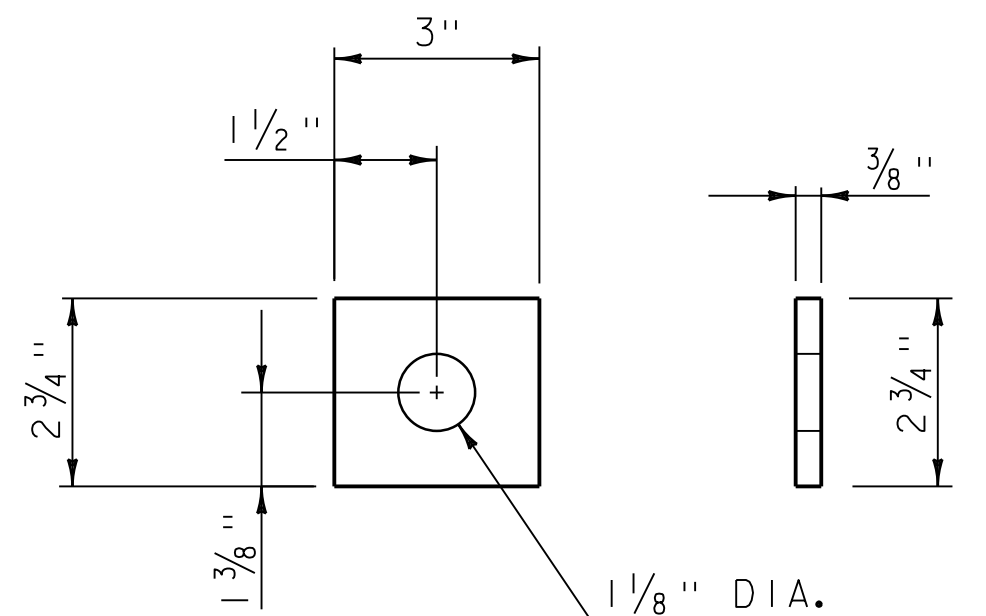
ANCHOR BRACKET END PLATE
