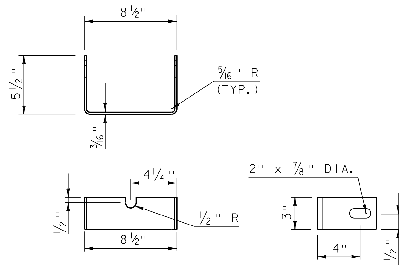
YOKE DETAIL
