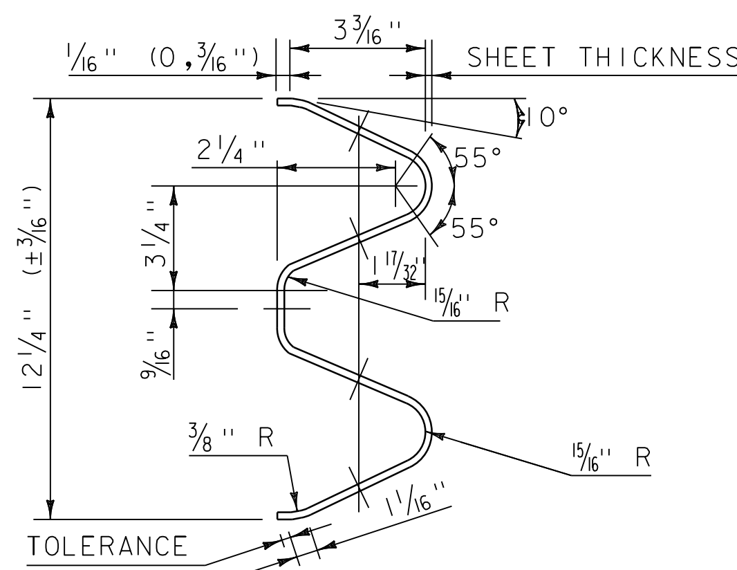
ARTBA RE-3 (2@6'-3"=12'-6" CLASS A, TYPE 1) - 73 TYPICAL GUARDRAIL SECTION
