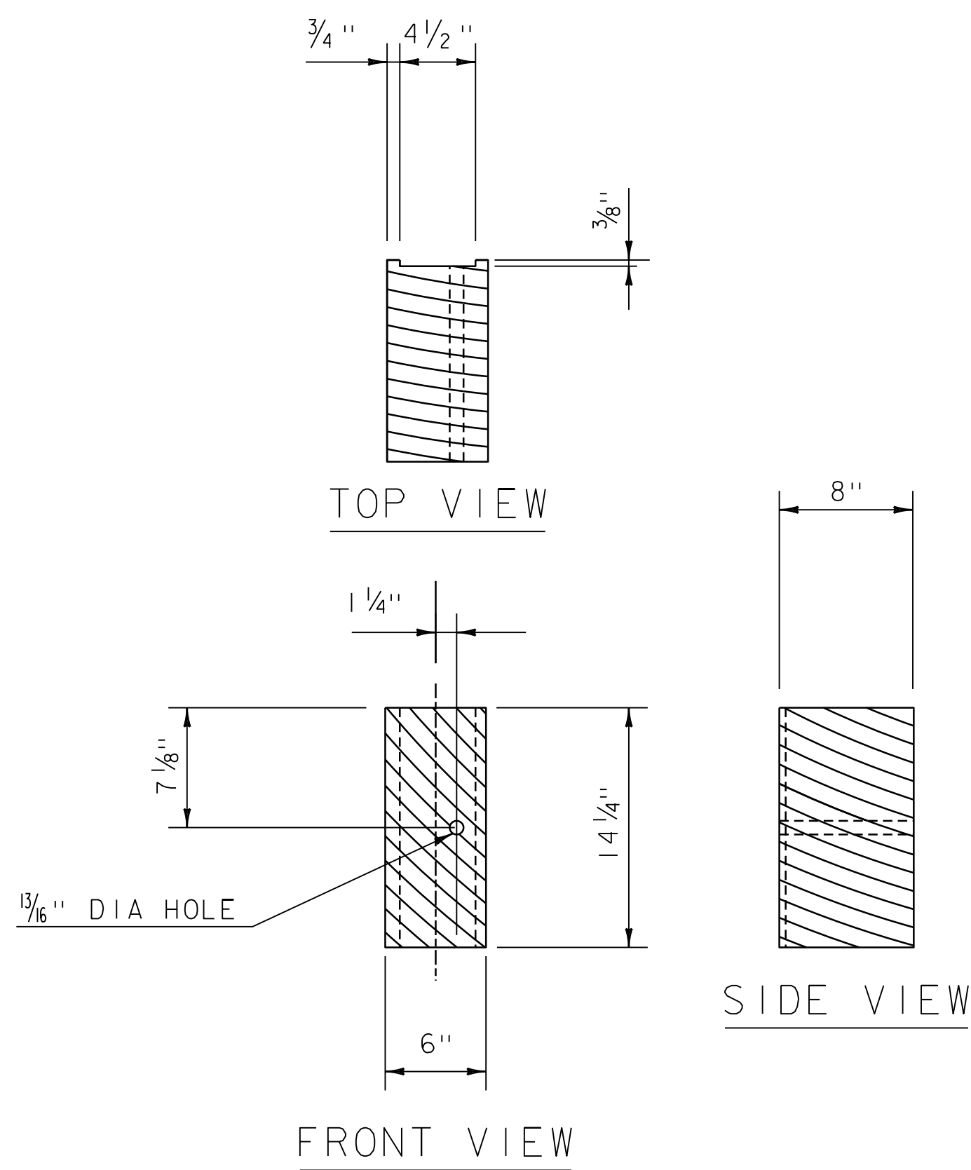
WOOD OFFSET BLOCK
