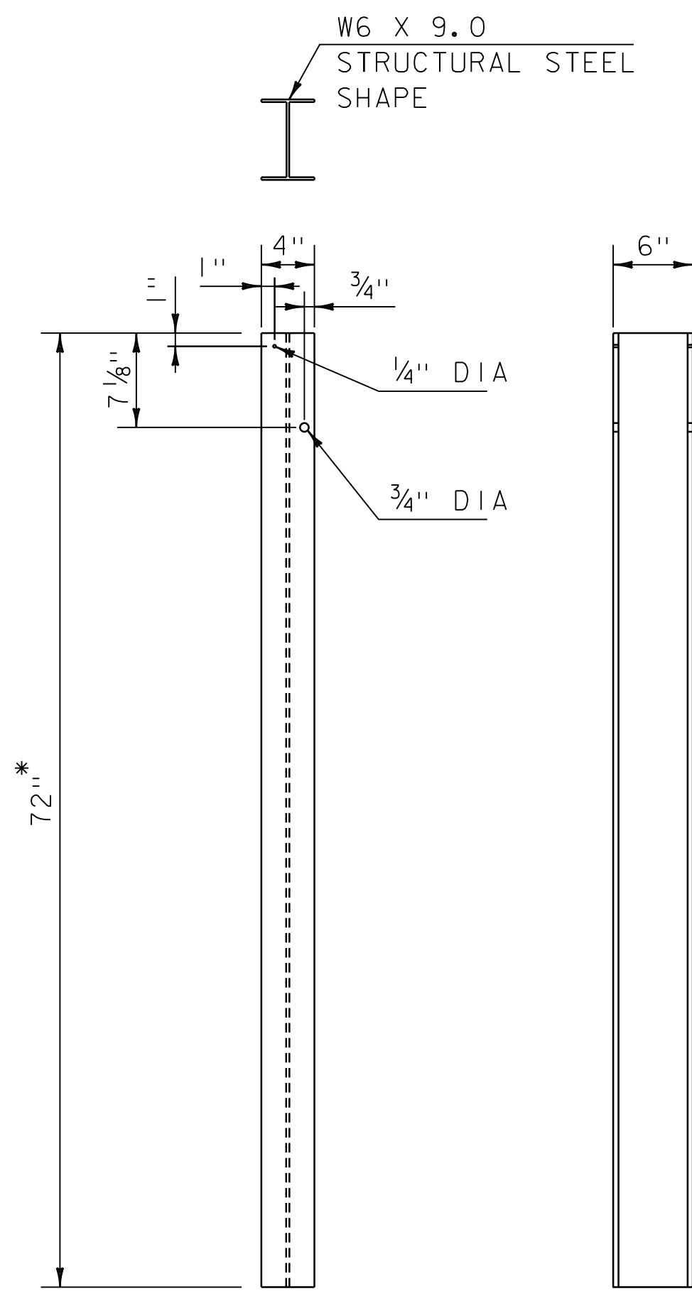
W6 X 9.0 STEEL POST
