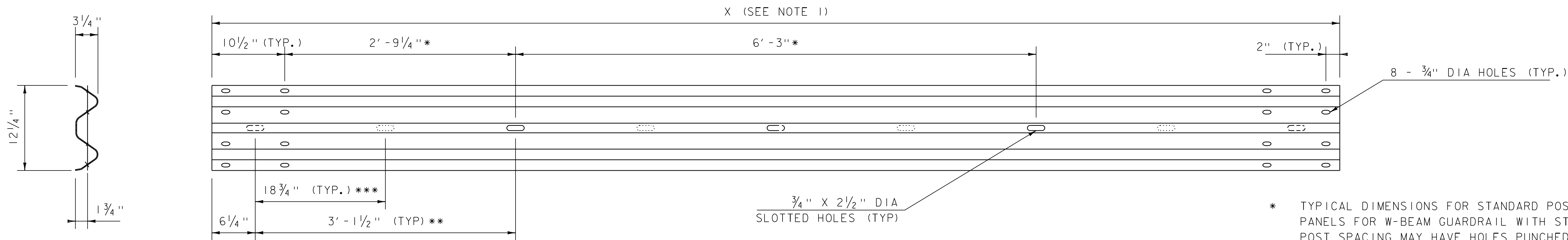
MGS GUARDRAIL
