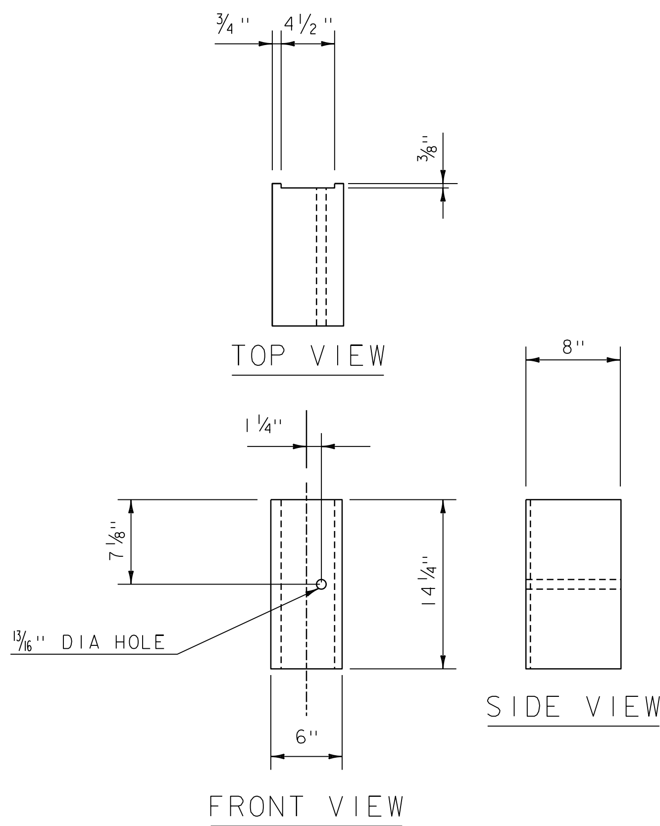
COMPOSITE OFFSET BLOCK
