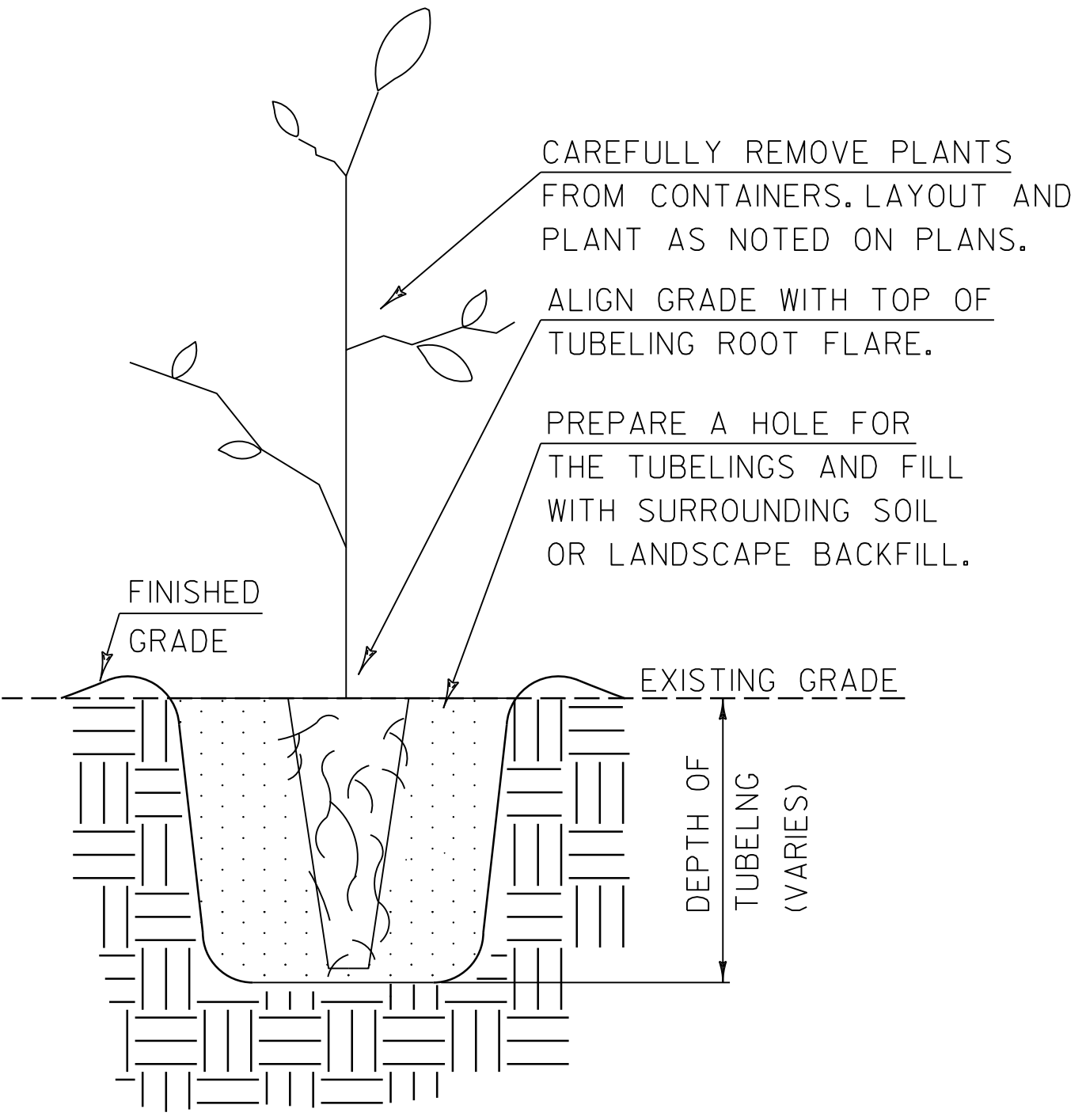
TUBELING PLANTING DETAIL
