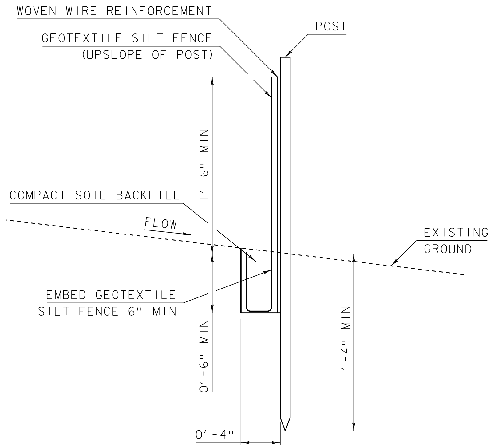
SECTION B-B
