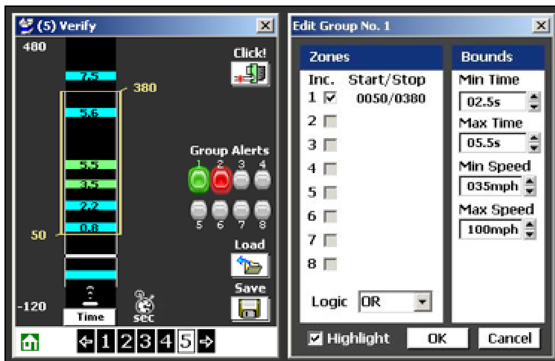
Figure 29 Manually established thresholds for Dilemma Zone
