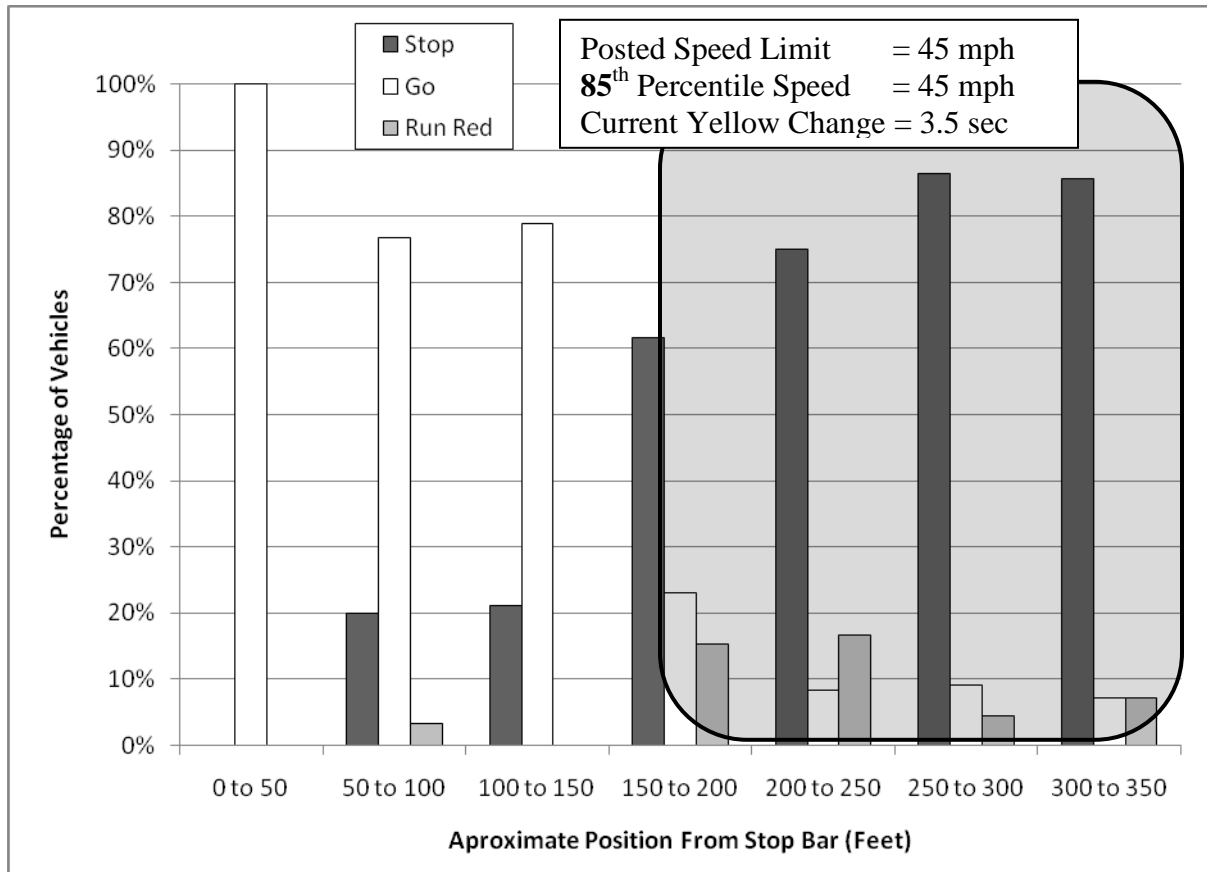
Figure 24 Relative Position and Driver Action of Vehicles at Onset of Yellow Indication Berlin Street @ Route 62 (Westbound Approach)
