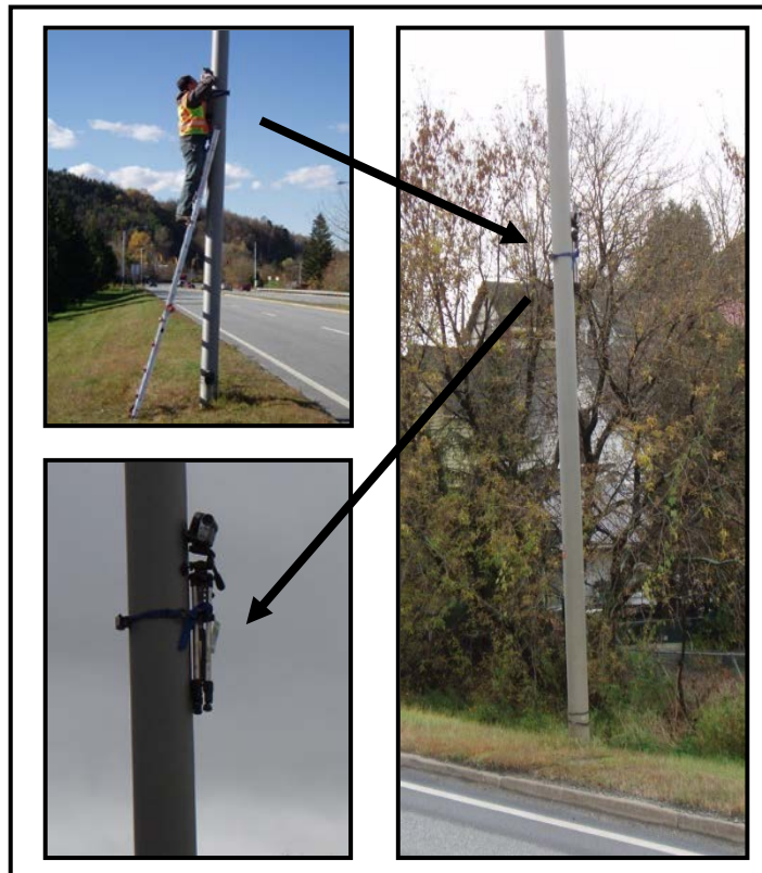
Figure 13 Example of Typical Video Camera Installation
