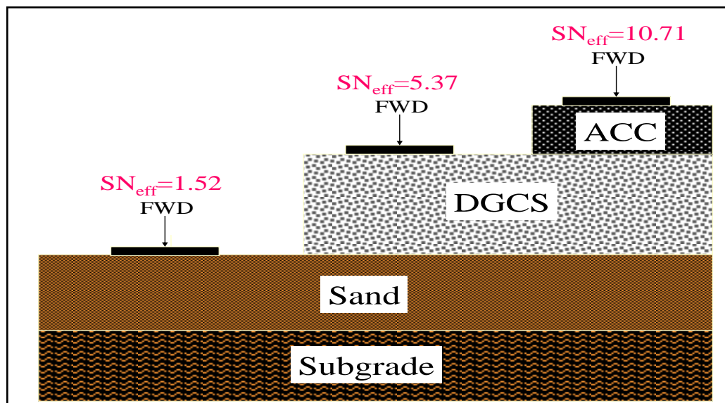
Figure 4 – FWD Testing Progression
