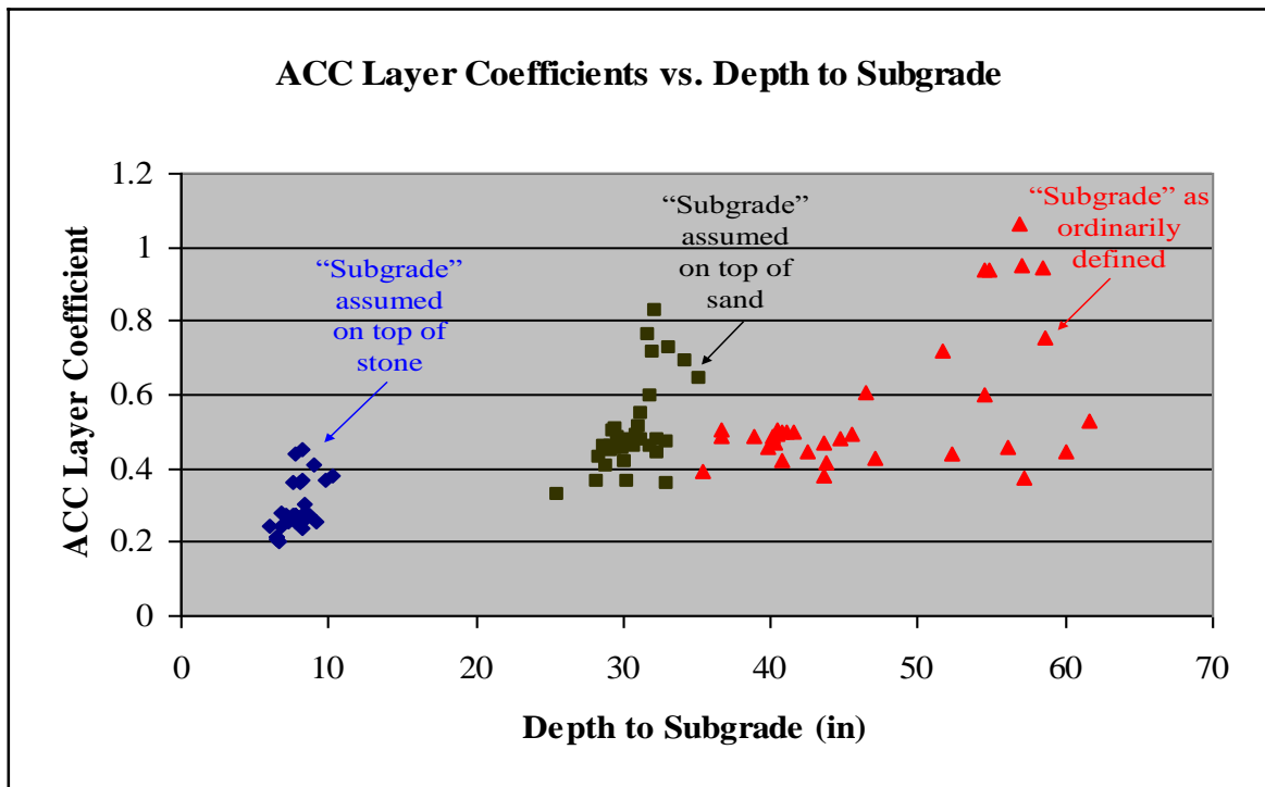
Figure 6 – ACC Layer Coefficient vs. Depth to Subgrade
