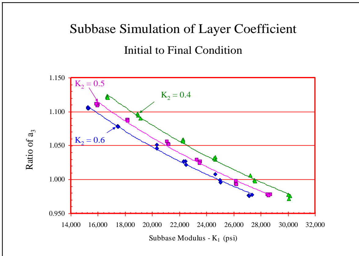
Figure 3 – Subbase Simulation of Layer Coefficient
