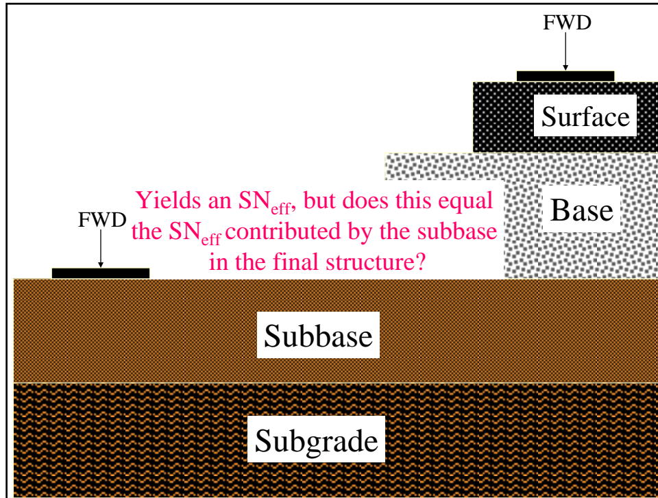
Figure 2 – Granular Subbase Behavior
