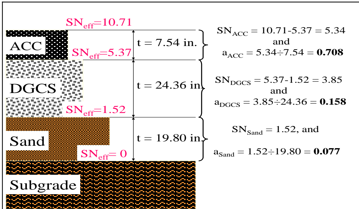
Figure 5 – Determination of Layer Coefficients from FWD Testing
